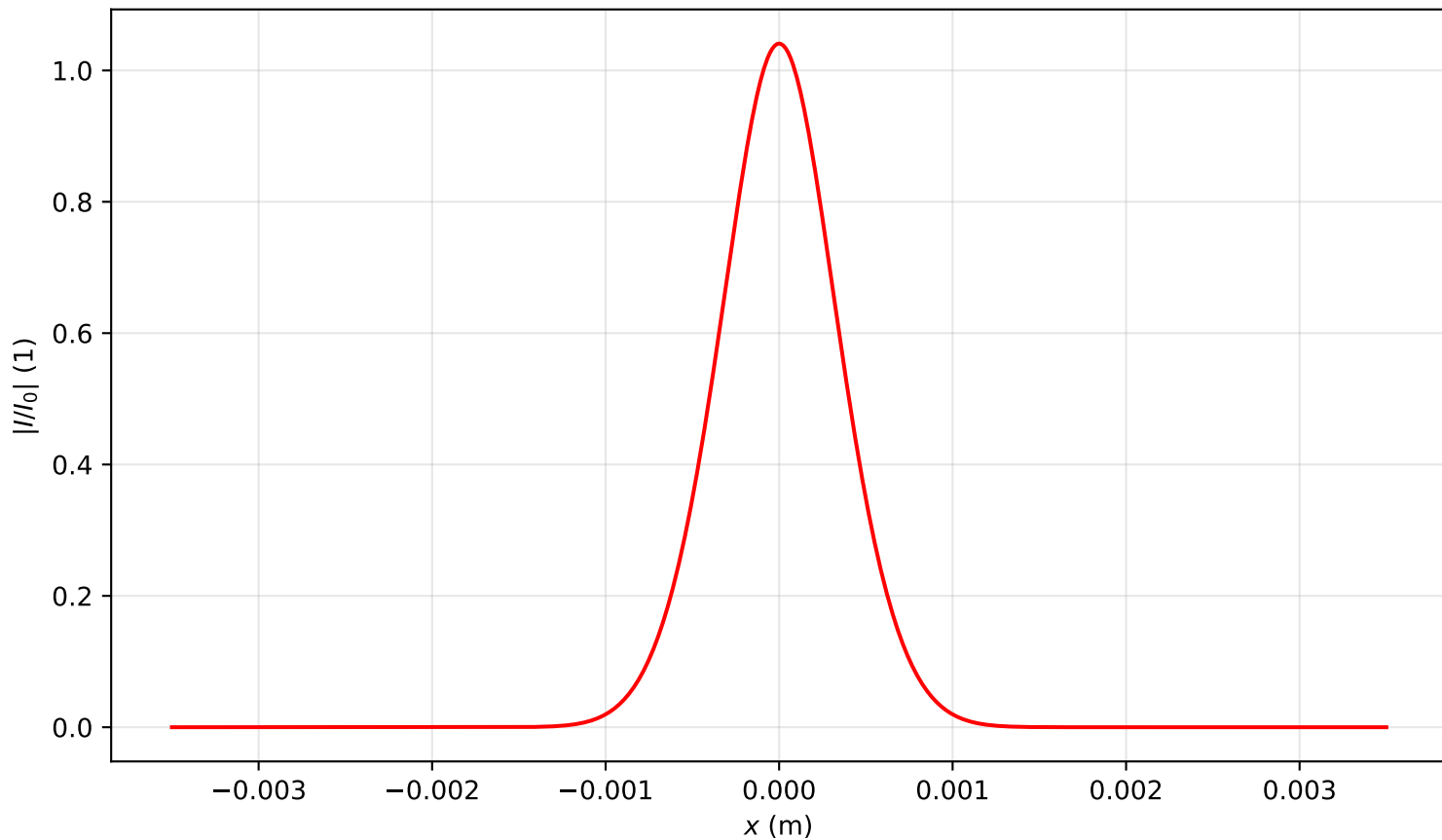
Intensity profile I(x, y = 0, z = 0.478)/I_0 , P_{in}=0.5P_{cr} , artificial time
